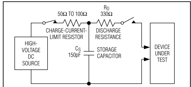
Figure 14. IEC 61000-4-2 Contact Discharge ESD Test Circuit
