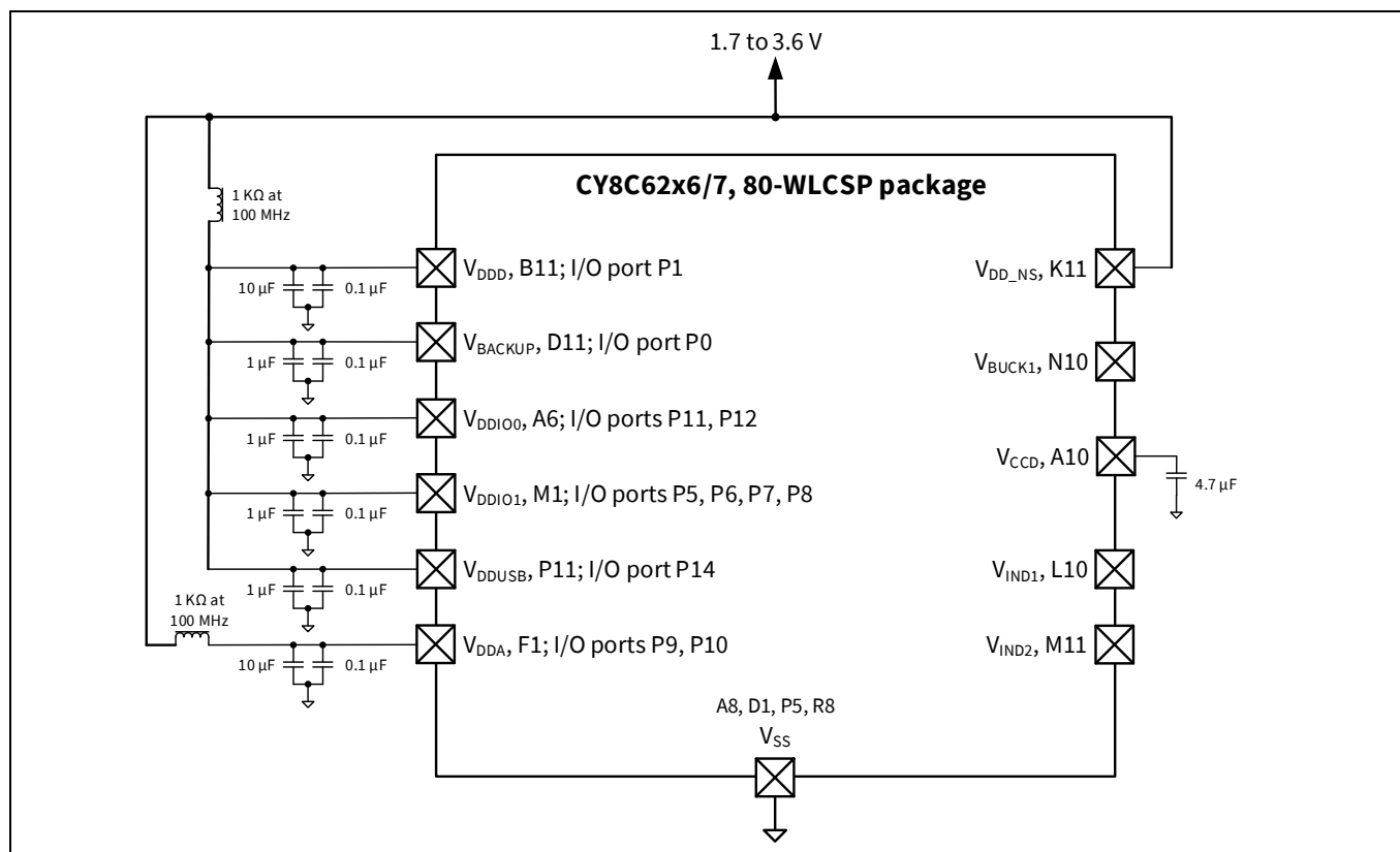
Figure 14 80-WLCSP (no buck) power connection diagram
