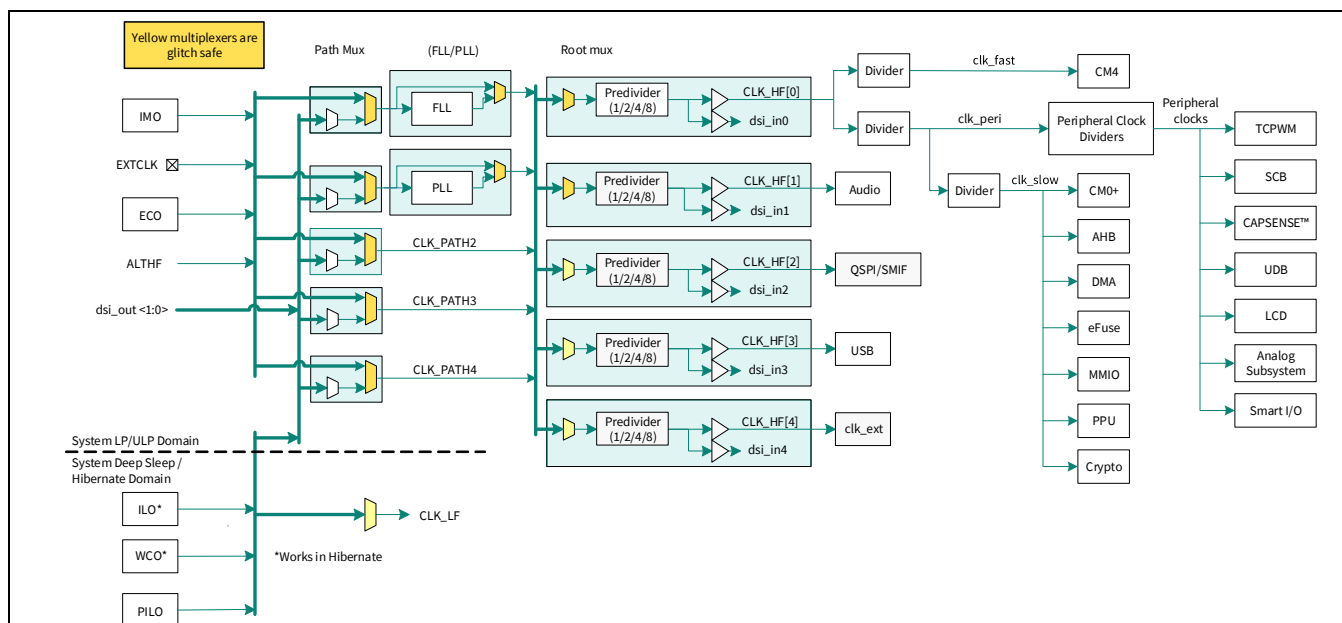
Figure 4 Clocking diagram
