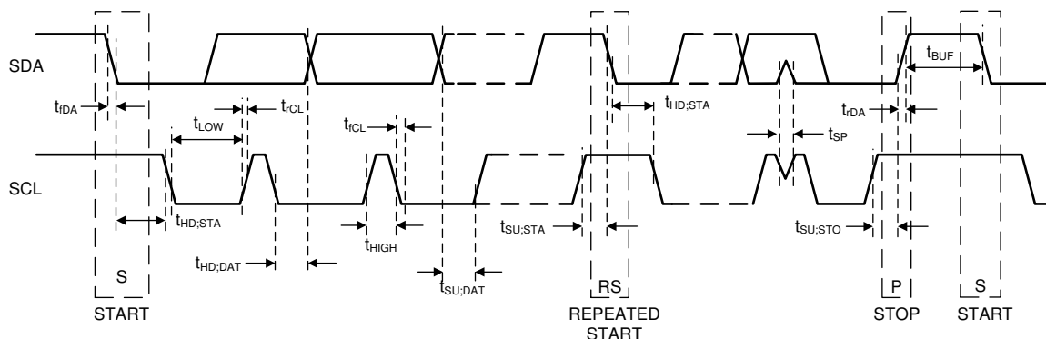
Figure 7-17. I²C-Compatible Timing
