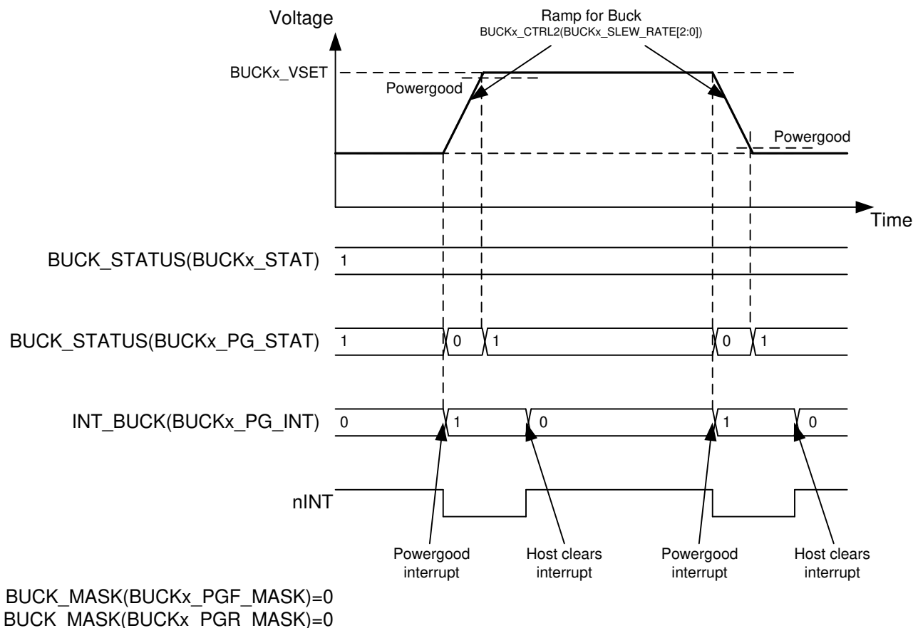
Figure 7-6. Buck Output Voltage Change
