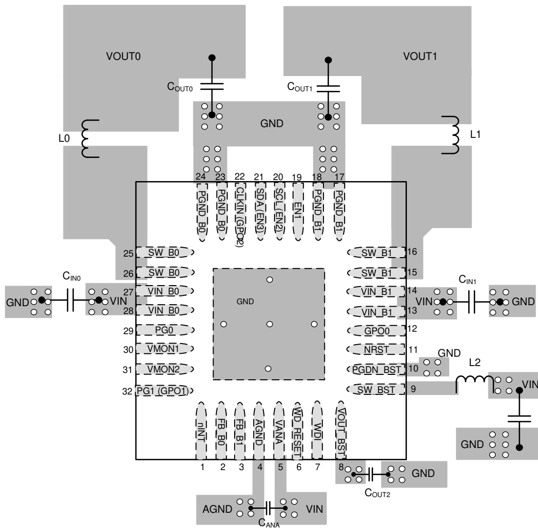
Figure 10-1. LP87702 Board Layout Example
