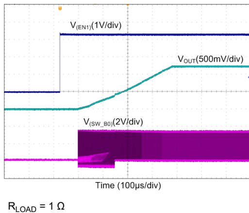
Figure 8-11. Buck Start-up with EN1, Forced-PWM
