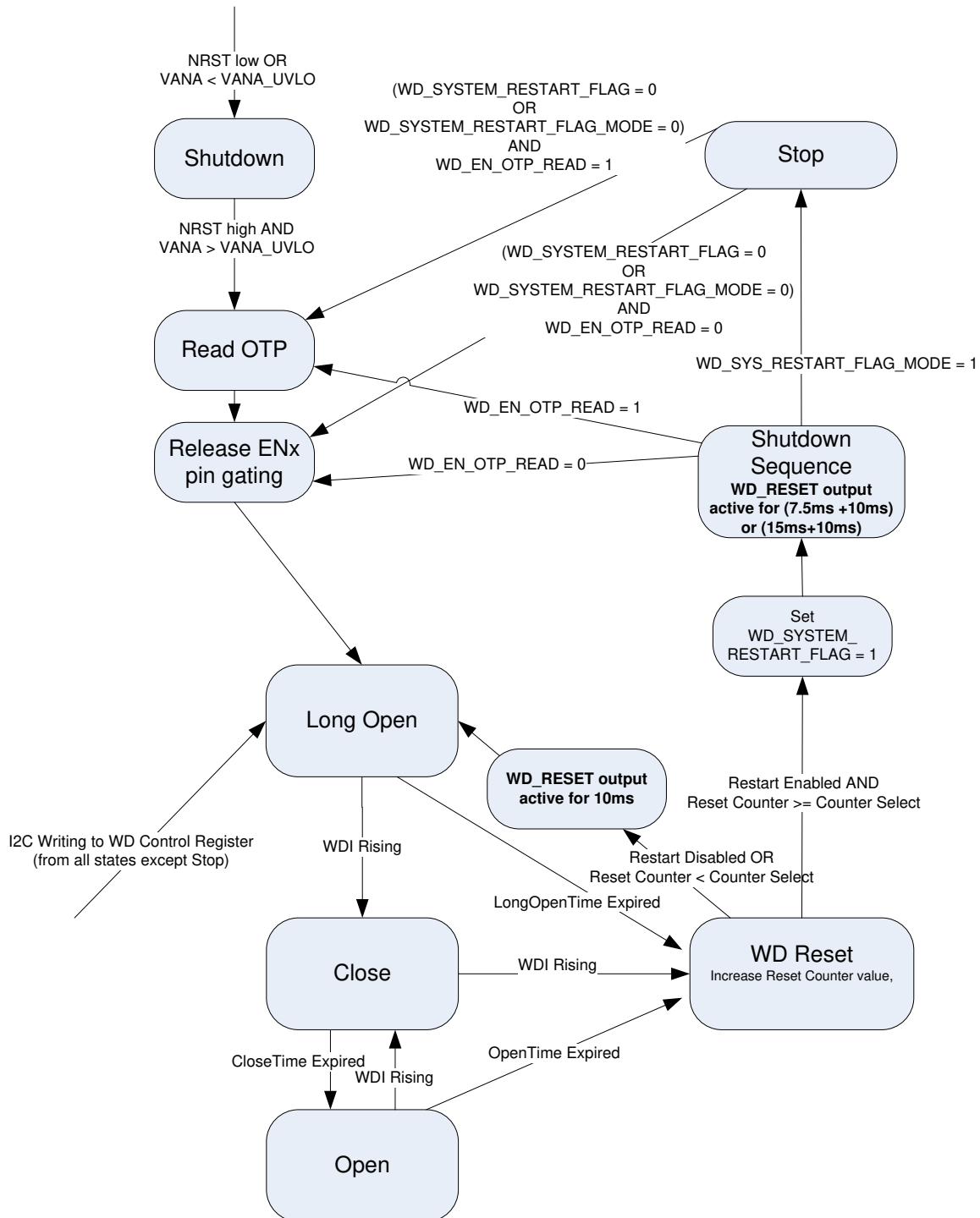
Figure 7-8. Watchdog Operation
