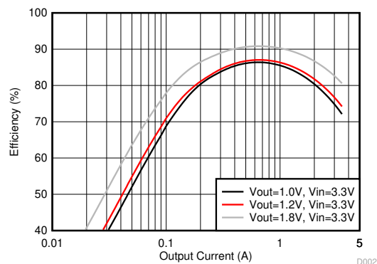
Figure 8-4. Buck Efficiency in Forced PWM Mode
