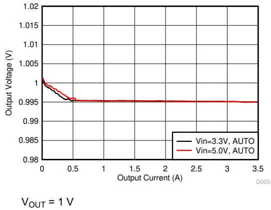
Figure 8-7. Buck Output Voltage vs Load Current in AUTO Mode
