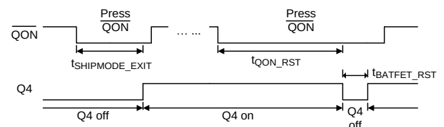
Figure 2. \overline{QON} Timing
