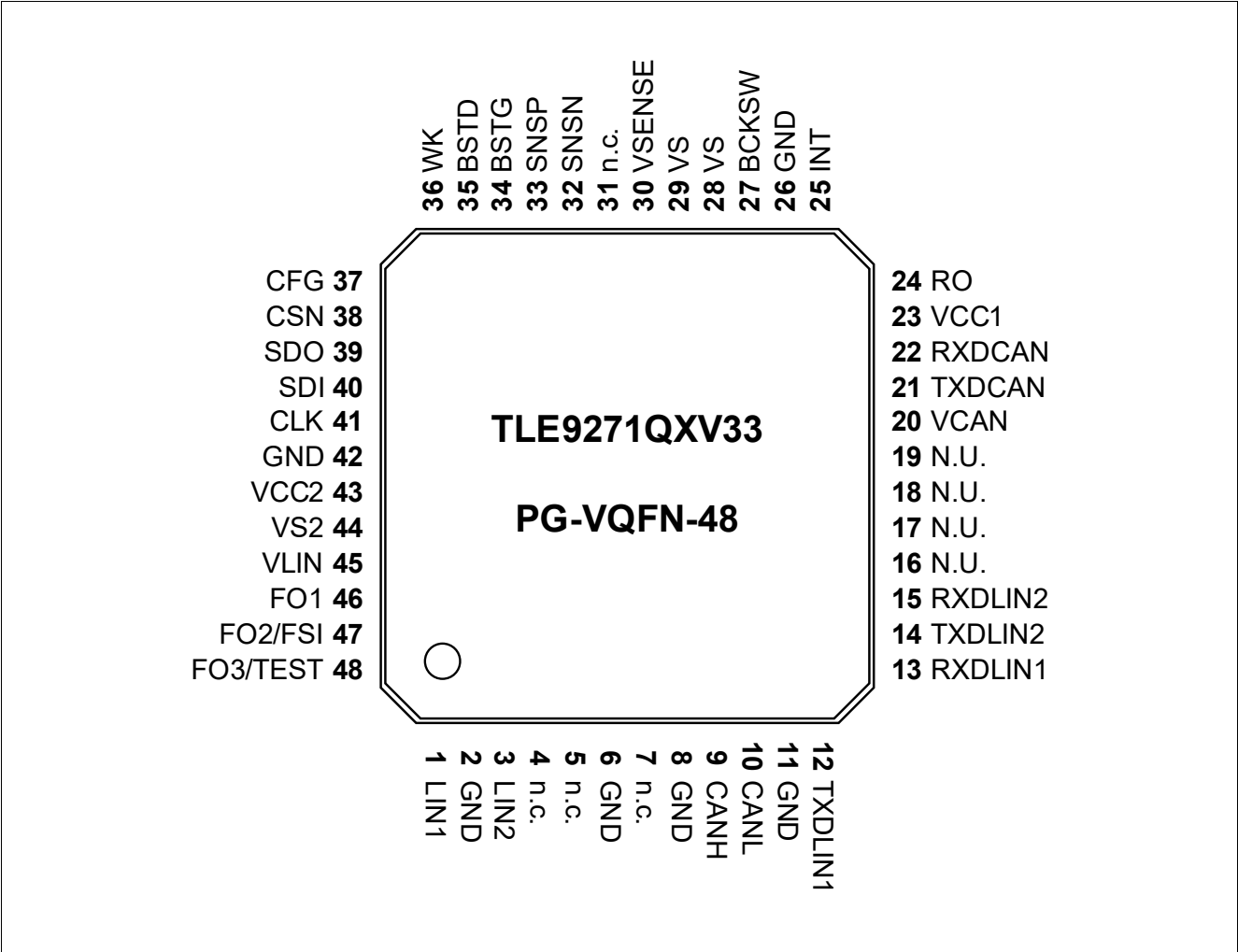
Figure 2 Pin assignment
