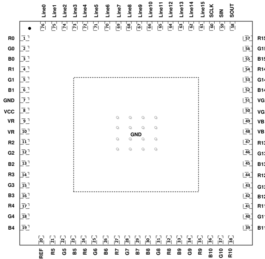
Figure 6-1. LP5890 RRF Package 76-Pin VQFN With Exposed Thermal Pad Top View
