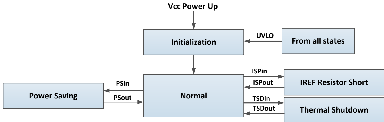
Figure 8-13. Functional Modes
