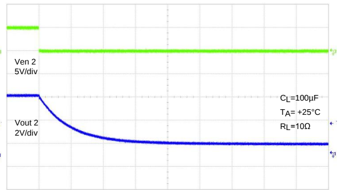
500μs/div Channel 2 Turn-Off Delay and Fall Time
