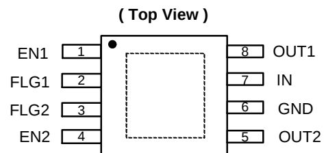
MSOP-8EP
