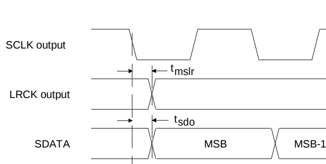
SCLK to SDATA & LRCK - MASTER Mode Serial Data Format, DFS low
