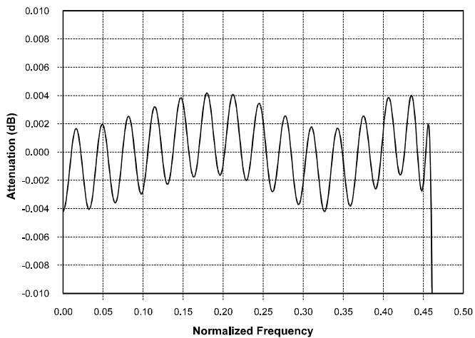
Figure 6. CS5394 Passband Ripple
