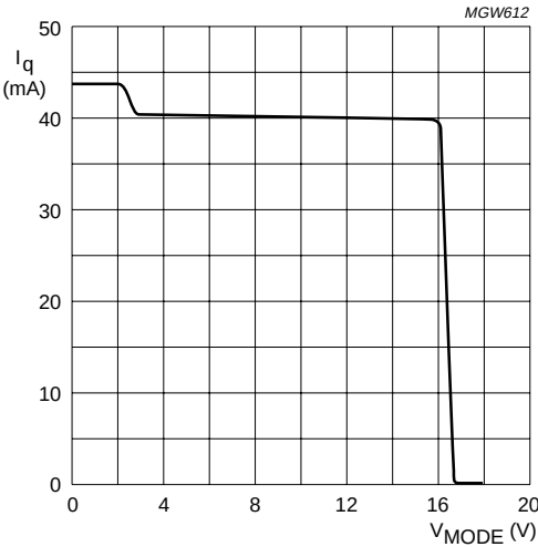
Fig 5. Quiescent current as function of mode voltage.
