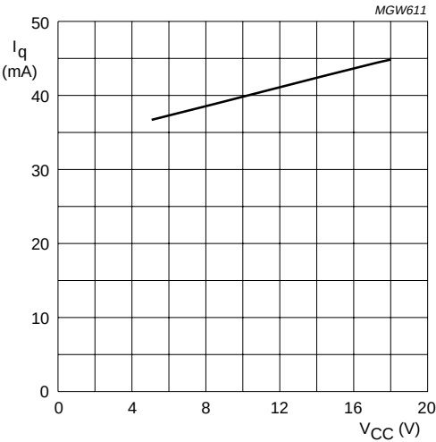
Fig 4. Quiescent current as function of supply voltage.
