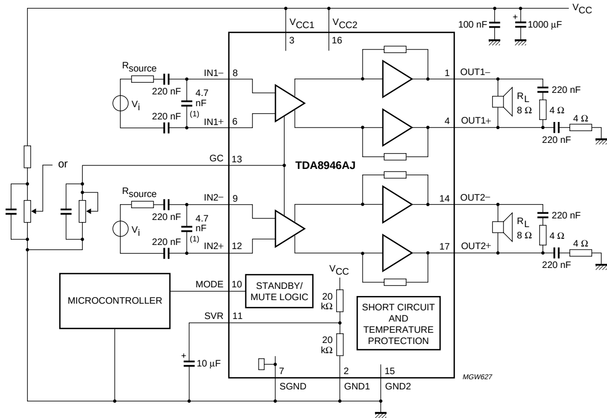
Fig 15. Application diagram.
