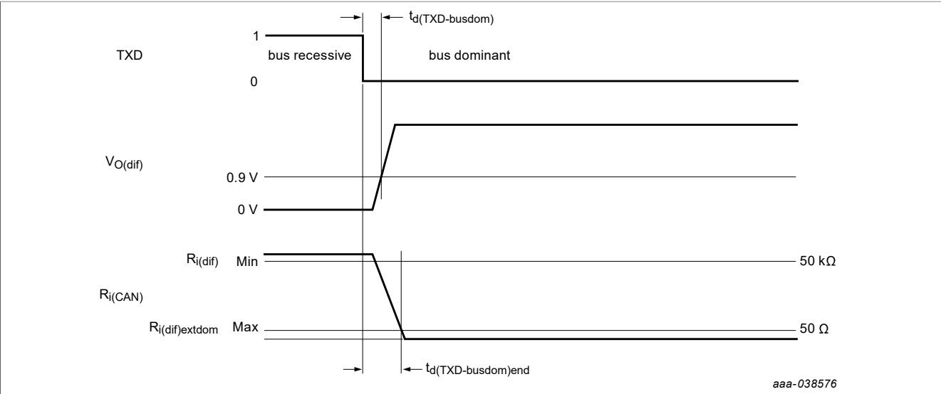
Figure 11. TJA1463 transmitter impedance and timing diagram for passive recessive-to-dominant transition
