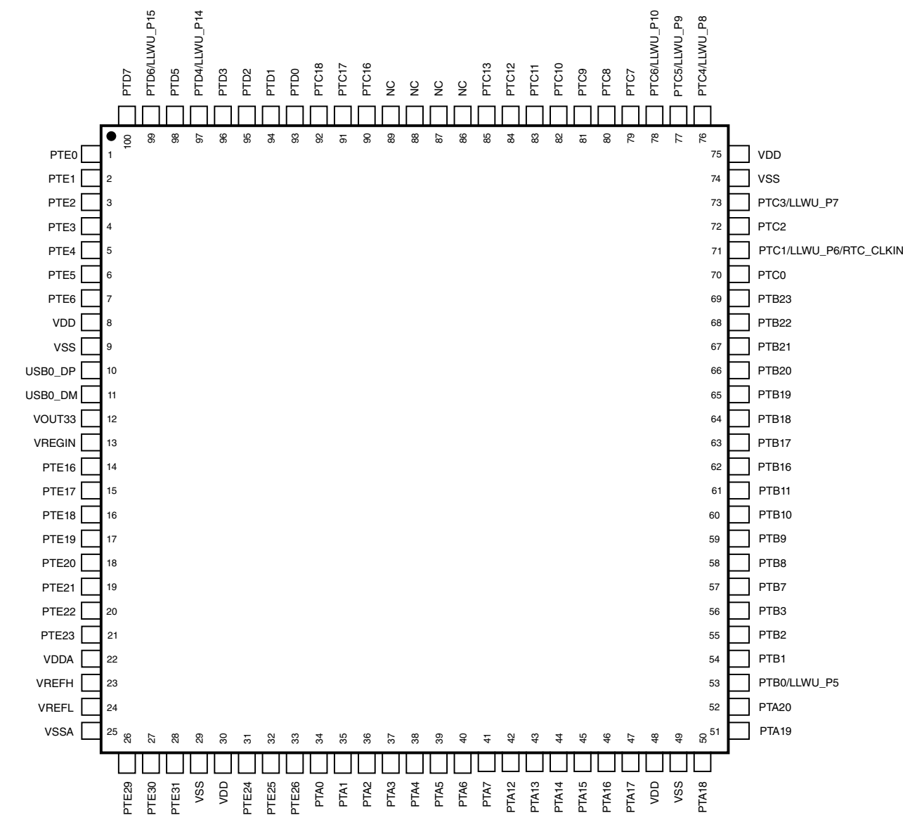
Figure 24. KL26 100-pin LQFP pinout diagram
