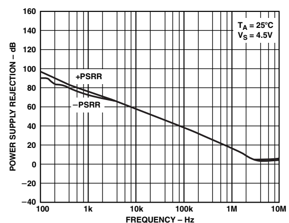
TPC 18. Power Supply Rejection Ratio vs. Frequency
