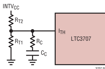
Figure 8. Active Voltage Positioning Applied to the LTC3707
