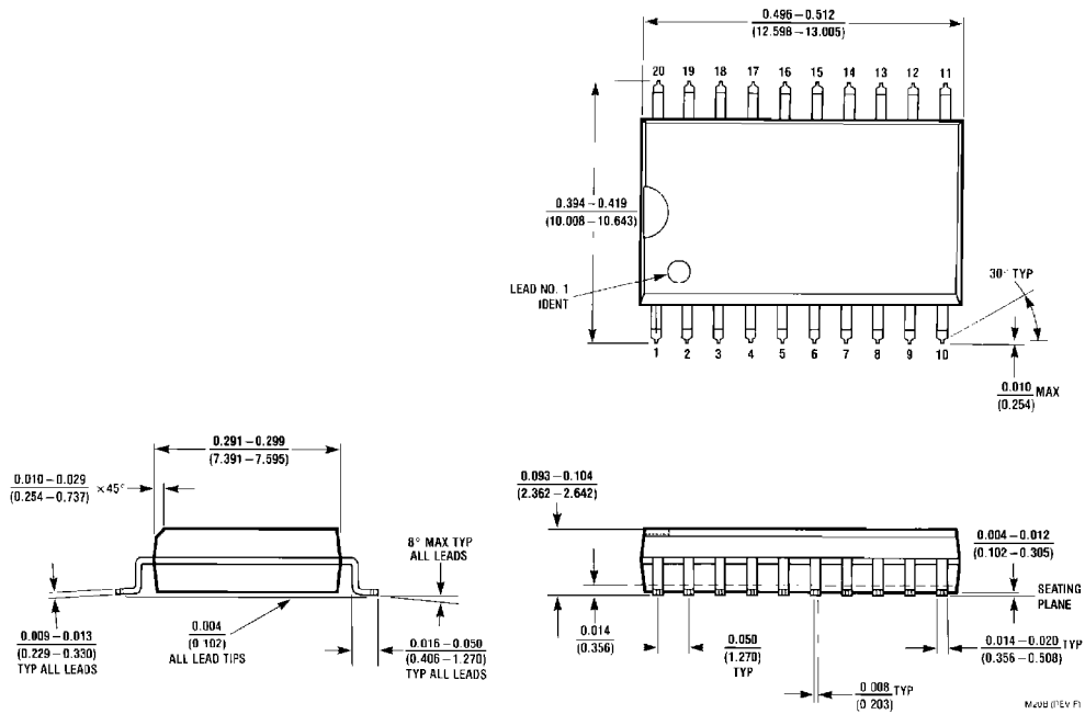
S.O. Package (M) Order Number DM74AL564AWM Package Number M20B
