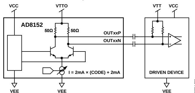
Figure 36. AC Coupling Output Signal from AD8152
