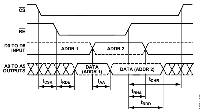
Figure 5. Second Rank Readback Cycle
