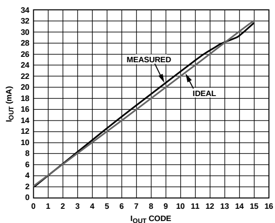
Figure 30. I_{OUT} vs. I_{OUT} Code
