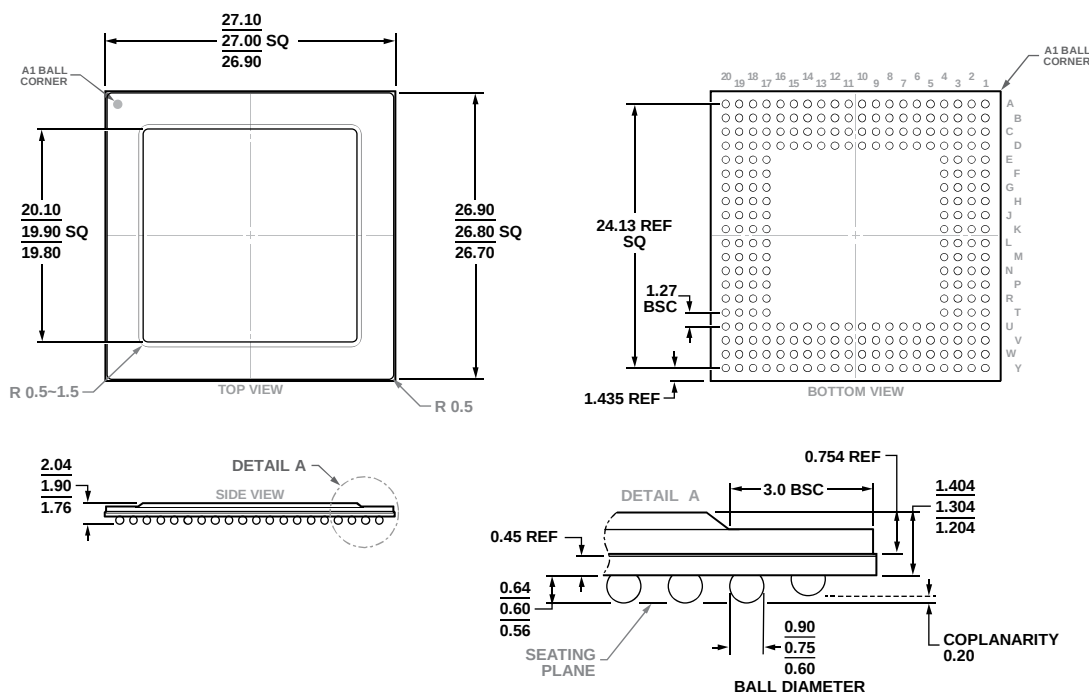
Figure 38. 256-Ball Ball Grid Array, Thermally Enhanced [BGA_ED] (BP-256-3)
