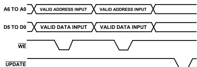
Figure 34. Programming Waveforms
