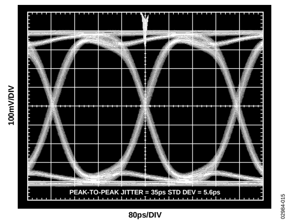
Figure 19. Crosstalk, 3.2 Gbps, Attack Signal Off (See Figure 33)
