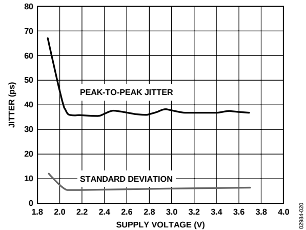
Figure 24. Jitter vs. Supply Voltage
