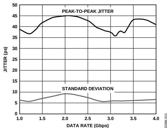
Figure 17. Jitter vs. Data Rate
