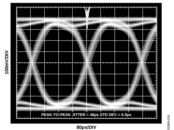
Figure 20. Crosstalk, 3.2 Gbps, Attack Signal On (See Figure 33)
