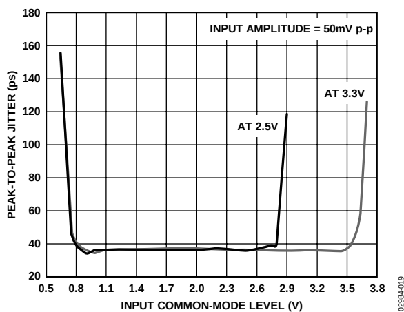
Figure 23. Peak-to-Peak Jitter vs. Input Common-Mode Level
