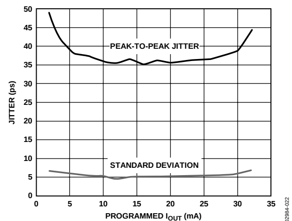
Figure 26. Jitter vs. Programmed I_{OUT}
