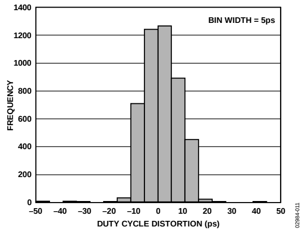
Figure 15. Duty Cycle Distortion Distribution
