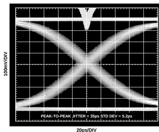
Figure 13. Jitter at 1.5 Gbps
