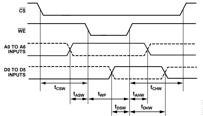
Figure 2. First Rank Write Cycle
