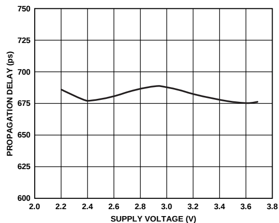
Figure 29. Propagation Delay vs. Supply Voltage
