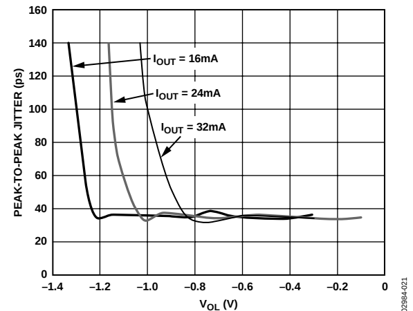
Figure 25. Peak-to-Peak Jitter vs. V_{OL} (Relative to VCC)
