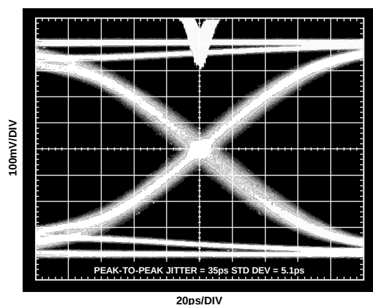
Figure 10. Jitter at 3.2 Gbps
