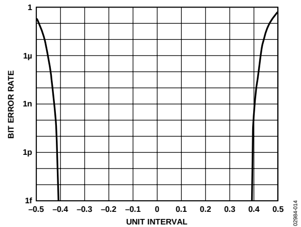
Figure 18. Bit Error Rate vs. Unit Interval
