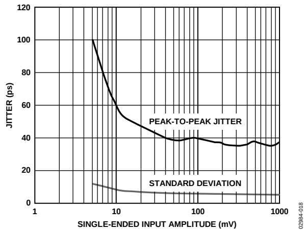
Figure 22. Jitter vs. Single-Ended Input Amplitude
