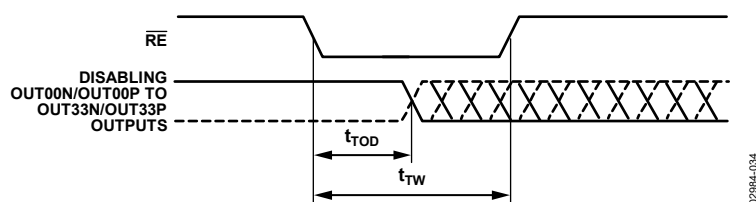
Figure 6. Asynchronous Reset
