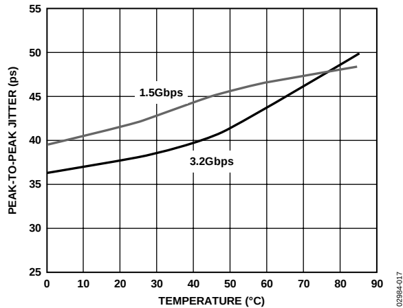
Figure 21. Peak-to-Peak Jitter vs. Temperature
