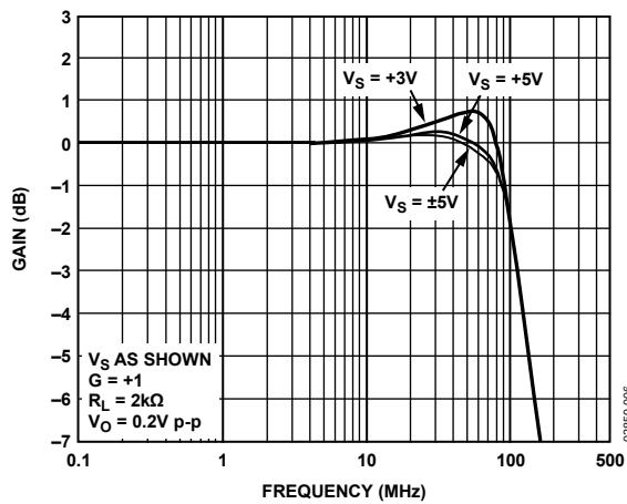
Figure 6. Gain vs. Frequency vs. Supply
