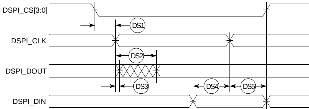
Figure 47. DSPI Timing
