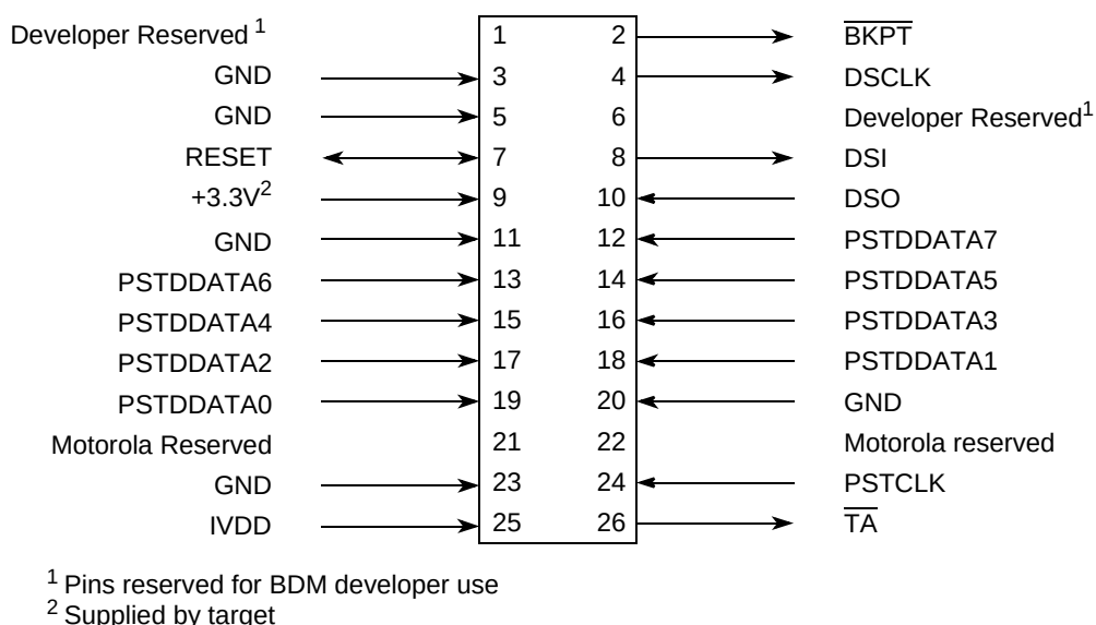
Figure 8. Recommended BDM Connector
