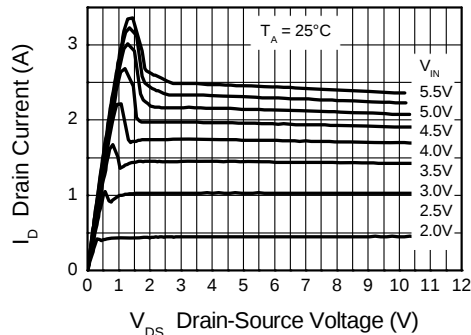
Typical Output Characteristic
