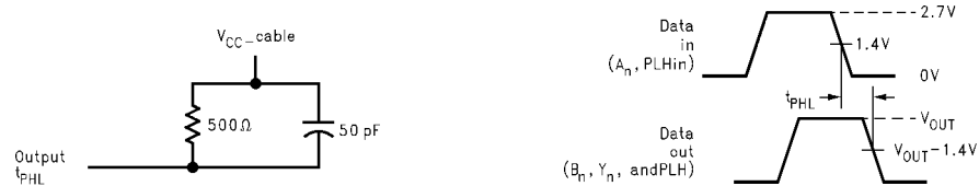
FIGURE 1. t_{PHL} Test Load and Waveforms
