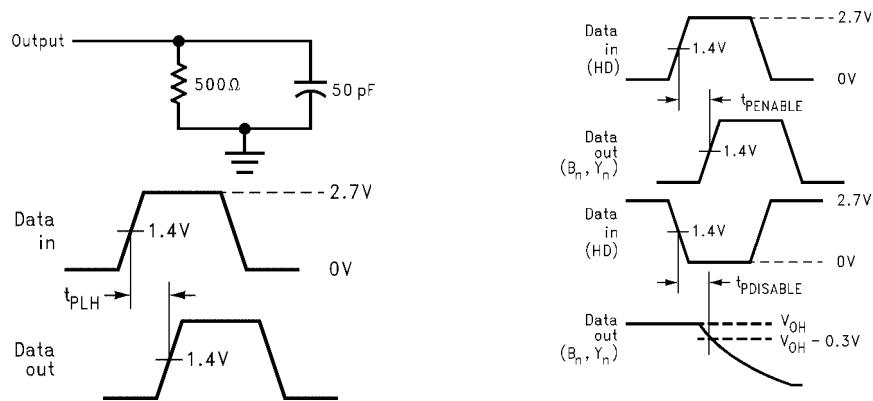
FIGURE 2. t_{PLH} , t_{pEn} , t_{pDis} Test Load and Waveforms
