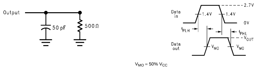
FIGURE 3. t_{PHL} , t_{PLH} Test Load and Waveforms
