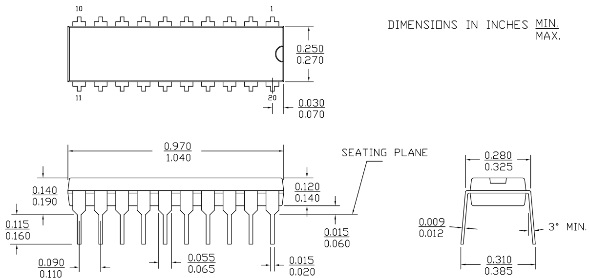
Figure 21. 20-Pin Molded DIP (300 Mils)
