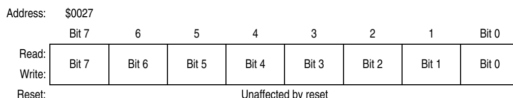
Figure 8-21. Pulse Accumulator Count Register (PACNT)
