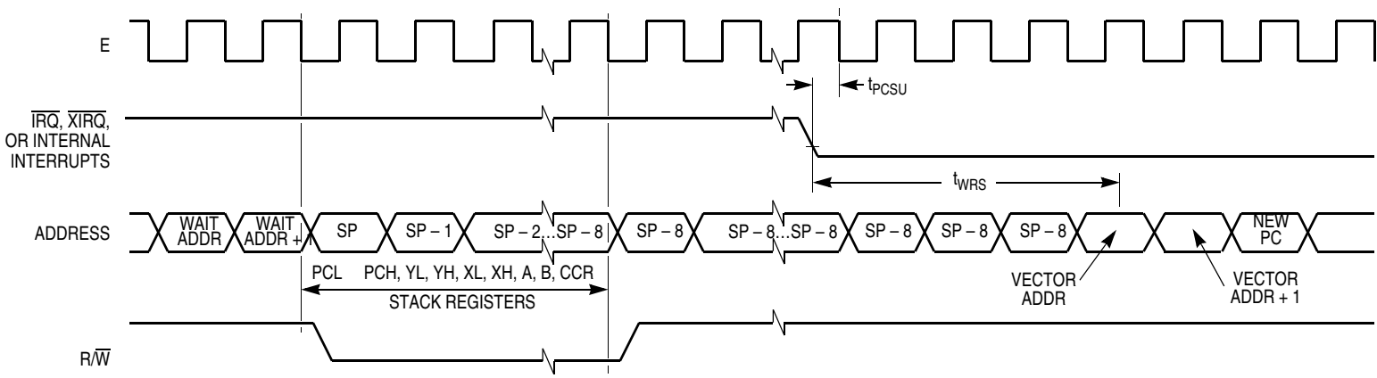
Figure 9-6. WAIT Recovery Timing Diagram
