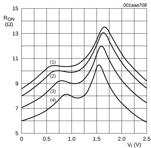
Fig 11. Typical ON resistance as a function of input voltage; T_{amb} = 25\text{ °C}
