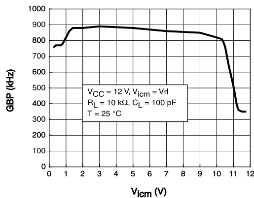
Figure 10. GBP vs. input common-mode voltage at V_{CC} = 12 V
