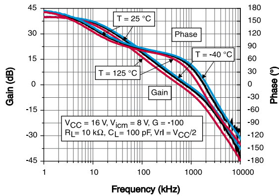
Figure 8. Bode diagram at V_{CC} = 16 V
