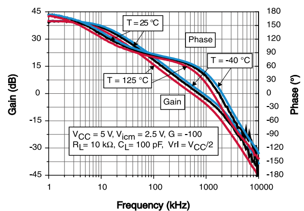
Figure 7. Bode diagram at V_{CC} = 5 V
