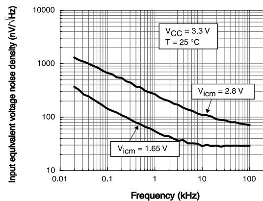
Figure 13. Noise vs. frequency at V_{CC} = 3.3 V
