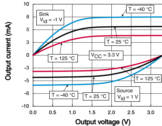
Figure 3. Output current vs. output voltage at V_{CC} = 3.3 V
