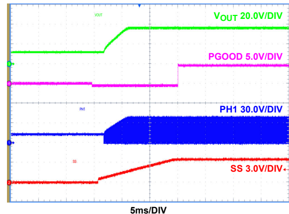
FIGURE 10. SOFT-START, DE+PHDROP MODE (DE/PHDRP = FLOAT), I_{OUT} = 8A
