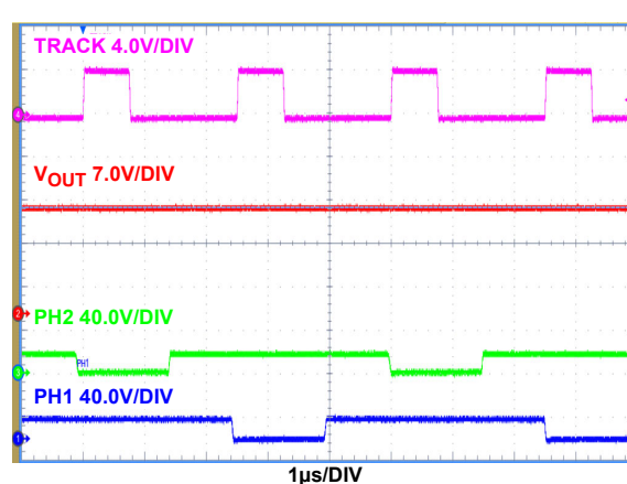
FIGURE 28. DIGITAL TRACKING (TRACKING SIGNAL, FREQUENCY = 400kHz, D_{TRACK} = 0.3 ), V_{OUT} = 17V
