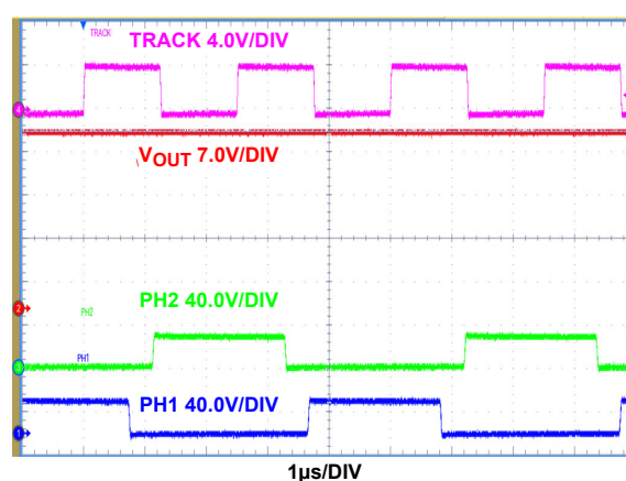
FIGURE 26. DIGITAL TRACKING (TRACKING SIGNAL, FREQUENCY = 400kHz, D_{TRACK} = 0.5 ), V_{OUT} = 28.3V
