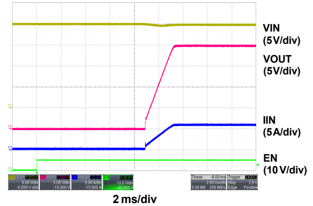
Figure 4. Soft-Start Delay ( V_{IN} = 20\text{V} , R_{OUT} = 3.4\Omega )
