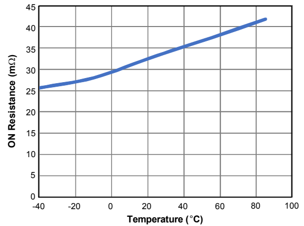
Figure 14. ON Resistance vs. Temperature (VIN=20V)
