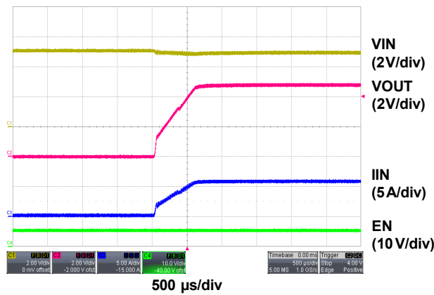
Figure 5. Soft-Start Ramp ( V_{IN} = 5\text{V} , R_{OUT} = 0.86\Omega )
