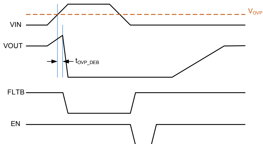
Figure 2. Over-Voltage Protection
