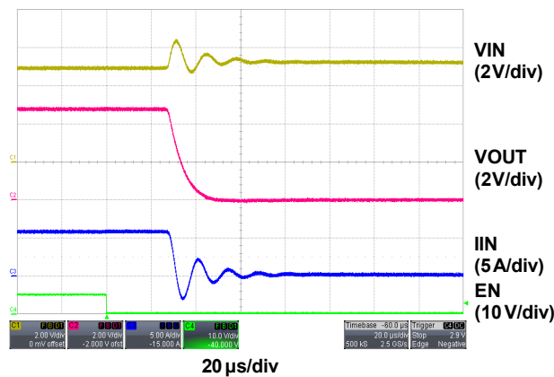
Figure 7. Shutdown ( V_{IN} = 5\text{V} , R_{OUT} = 0.86\Omega )
