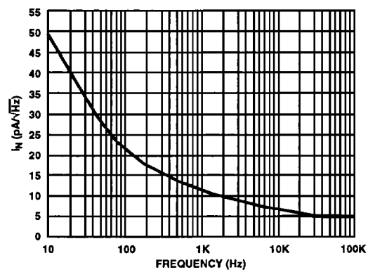
FIGURE 8. NOISE CURRENT vs FREQUENCY V_{\text{CC}} = \pm 15\text{V}
