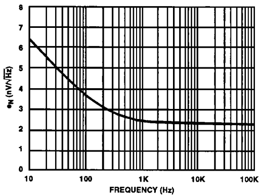
FIGURE 7. NOISE VOLTAGE vs FREQUENCY V_{\text{CC}} = \pm 15\text{V}
