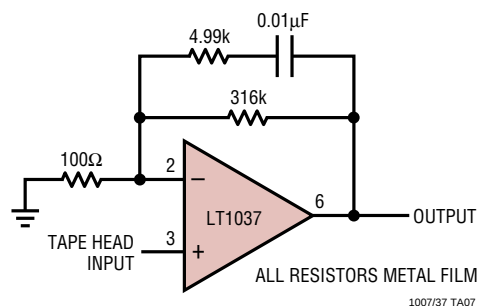
Tape Head Amplifier
