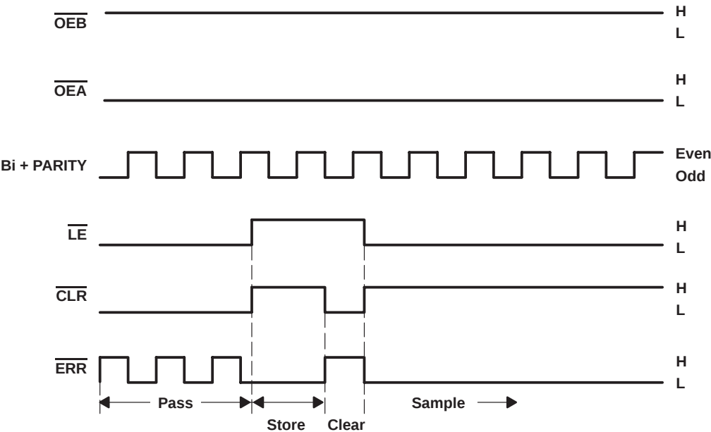
ERROR-FLAG FUNCTIONS
