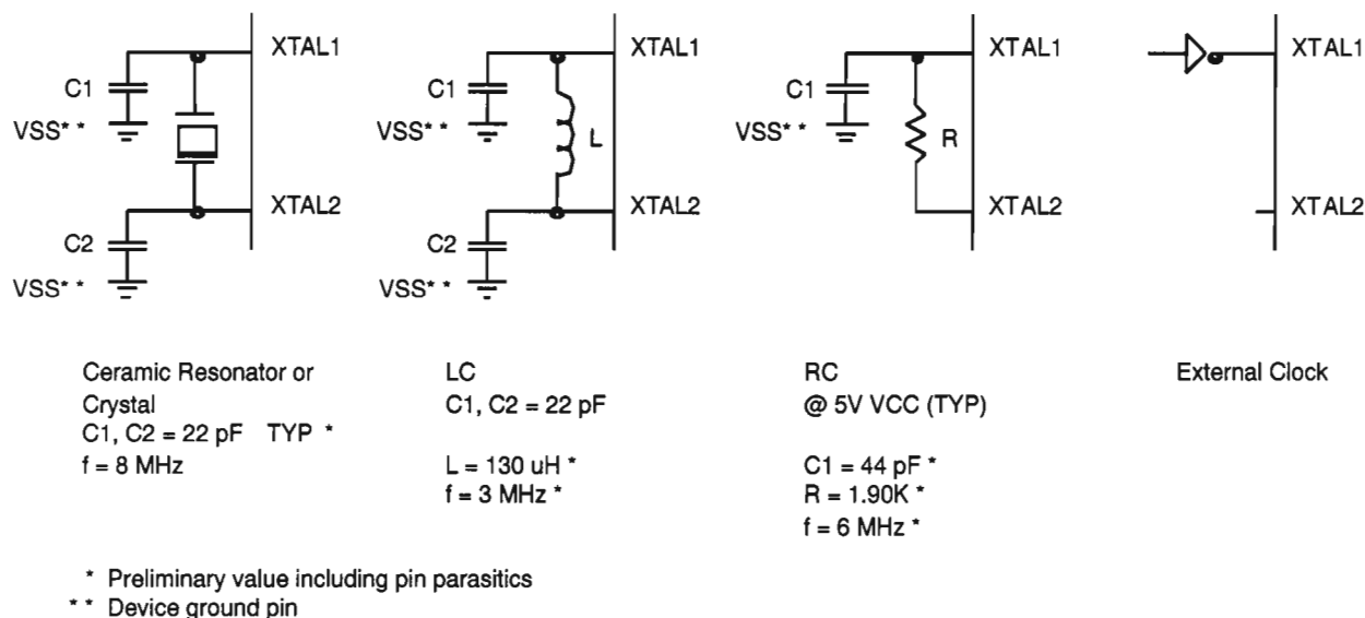
Figure 24. Oscillator Configuration
