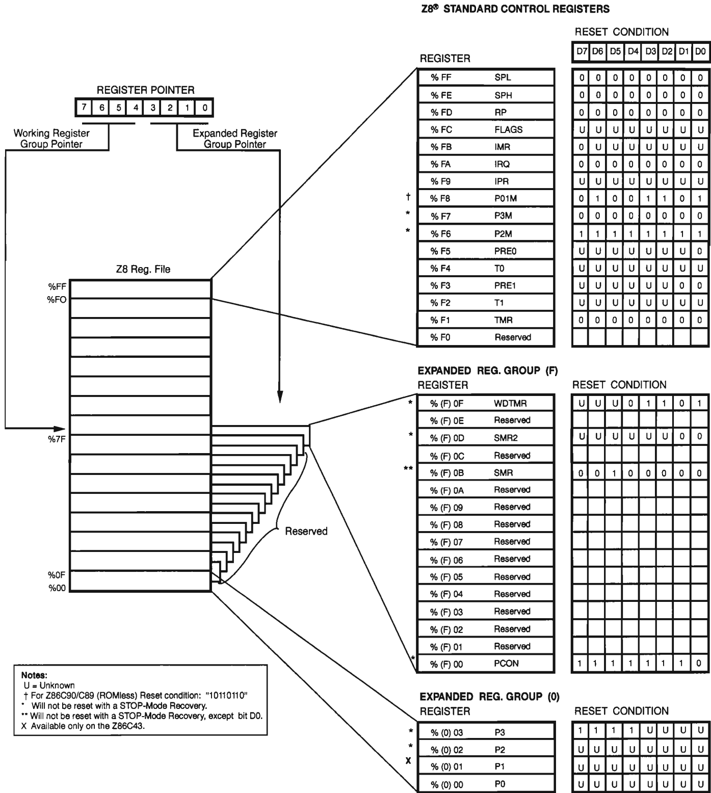
Figure 19. Expanded Register File Architecture
