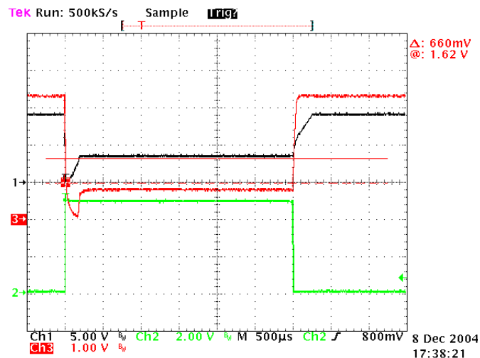
FIGURE 18. WOC OPERATION
