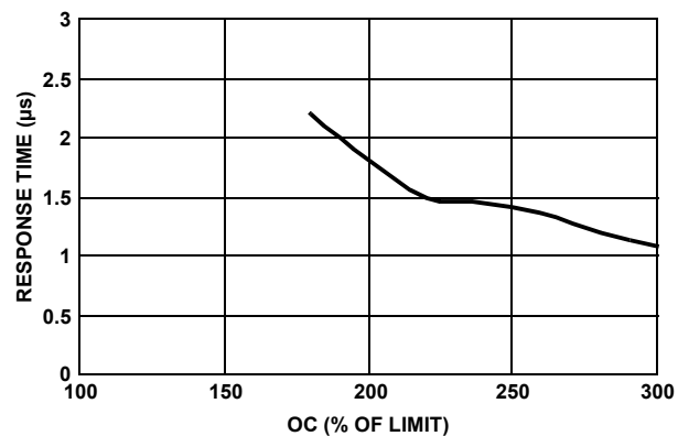
FIGURE 10. RESPONSE TIME vs I_O \cdot R_{SNS}
