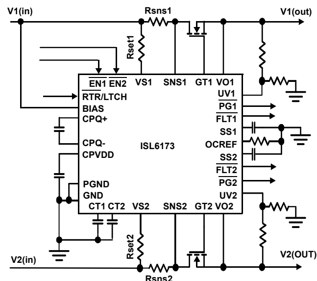
FIGURE 1. TYPICAL APPLICATION
