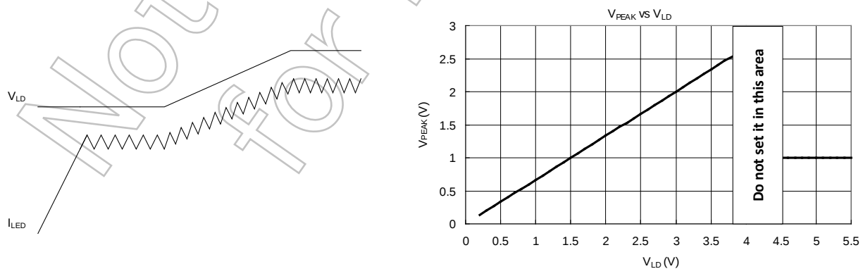
(a) Waveform of LED current vs control voltage V_{LD}
