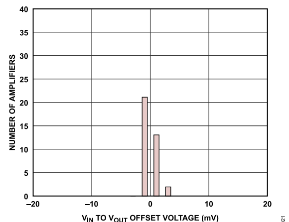
Figure 21. V_{IN} to V_{OUT} Offset-Voltage Distribution at 25^{\circ}\text{C} , Output Offset-Voltage for V_{IN} = 2.5\text{ V}
