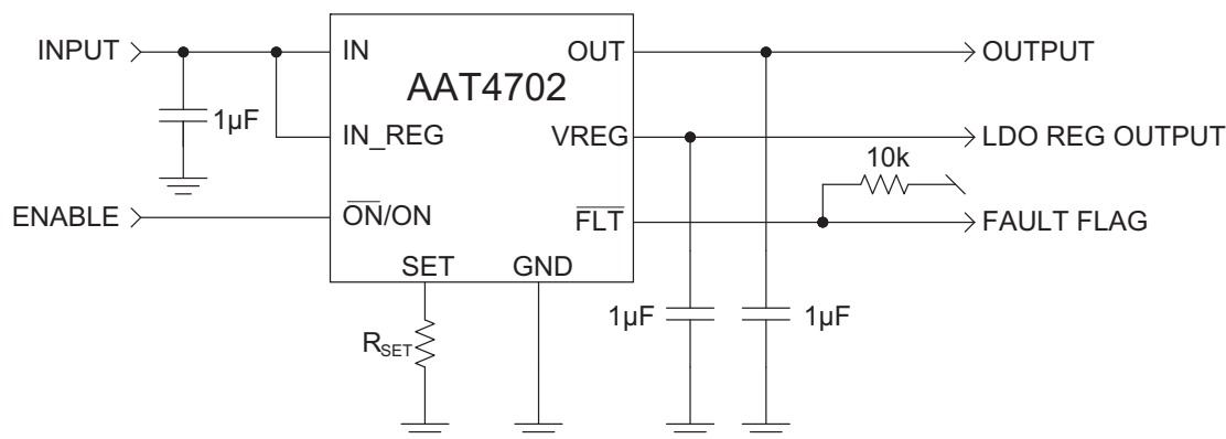
Figure 3: AAT4702 Application Circuit with User Set ( R_{\text{SET}} ) Current Limit and Fault Flag Pull-Up Resistor.
