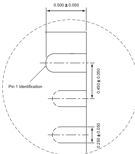
Detail "A"
