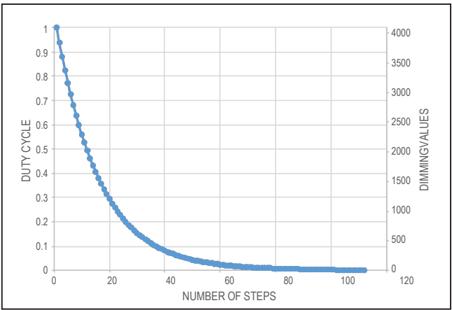
Figure 4. Down-Transition Curve
