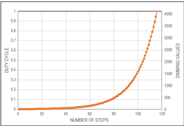
Figure 3. Up-Transition Curve
