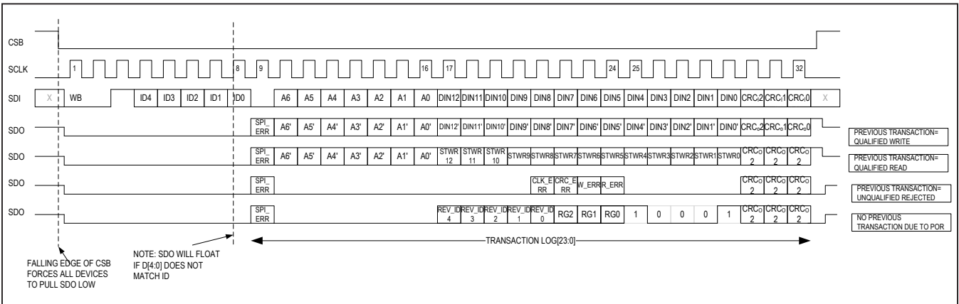
Figure 8. Write-Mode Transaction
