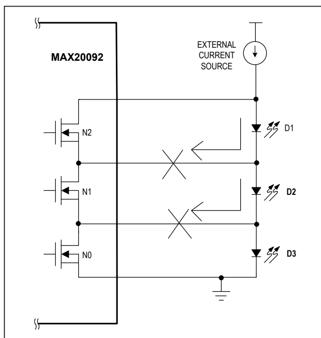
Figure 1. Open-Trace Detection
