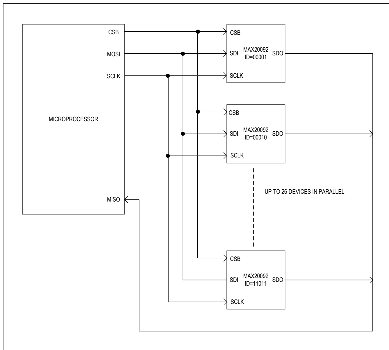
Figure 7. Star Connections
