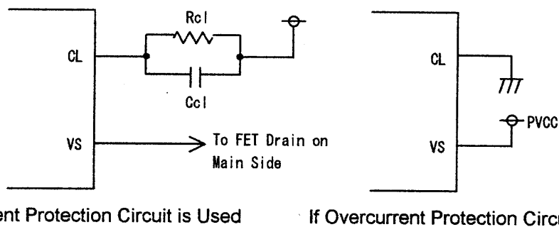
Figure - 11 CL and VS Terminal Connections
