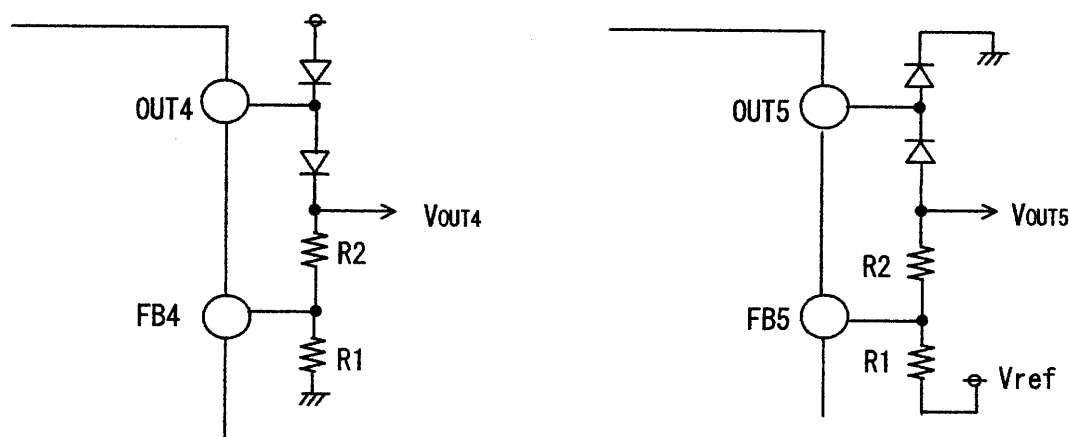
Figure - 15 Setting Output Voltage For OUT4,5
