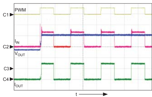
50% Duty Cycle
