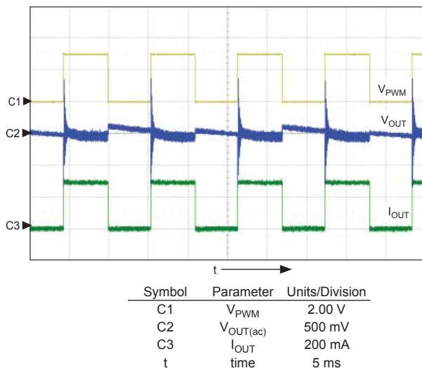
Figure 3. Output Voltage Ripple During PWM Dimming. V_{IN} = 5 V, V_{BAT} = 15 V, f_{SW} = 1 MHz, f_{PWM} = 100 Hz, PWM duty cycle = 50%, 8S8P configuration, 40 mA per channel.
