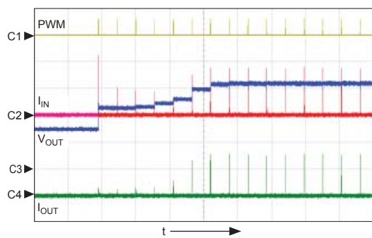
1% Duty Cycle
