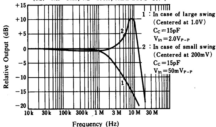
Reference Input Frequency Respons
