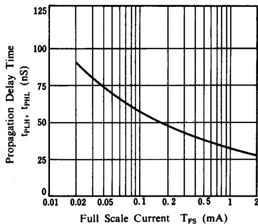
Propagation Delay Time vs. Full Scale Current
