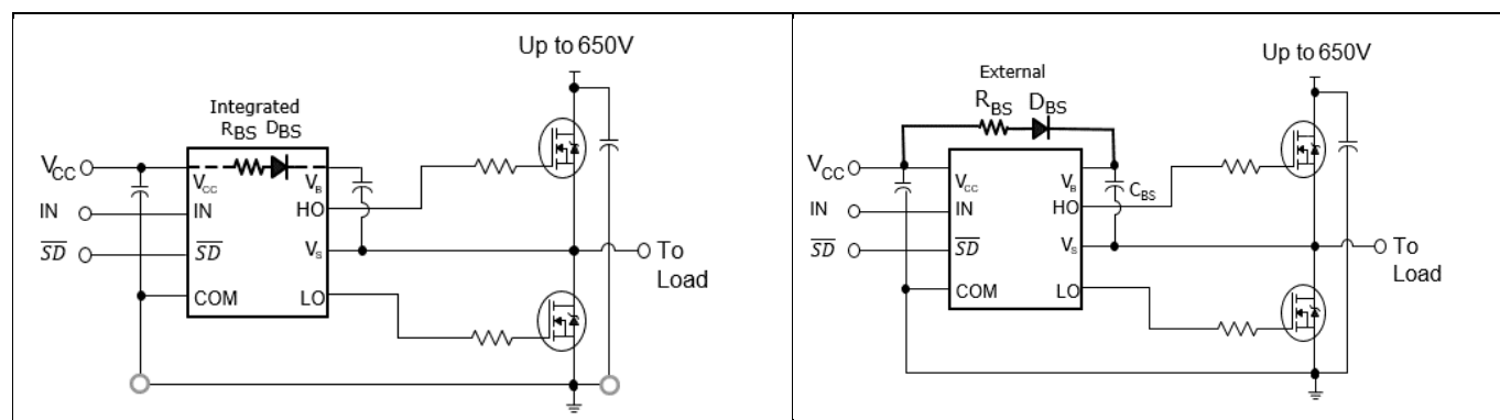
Figure 13 2ED210x with integrated components Figure 14 Standard bootstrap gate driver
