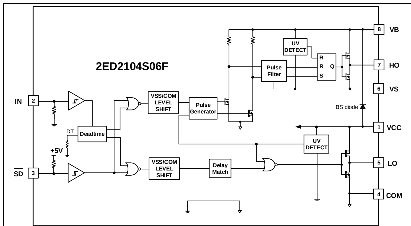
Figure 2 Block diagrams
