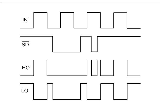
Figure 7 Input/output logic diagram
