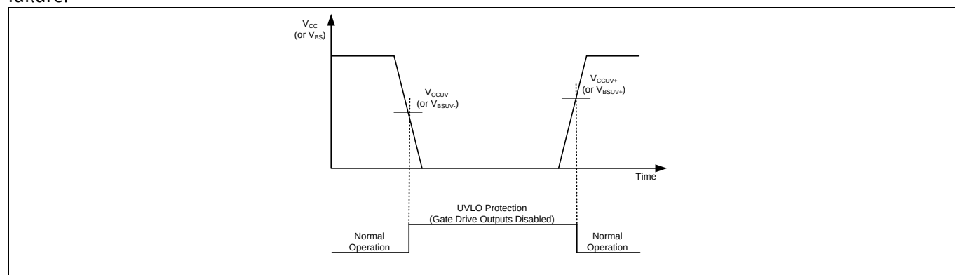
Figure 12 UVLO protection
