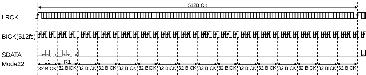
Figure 40. Mode 22 Timing
