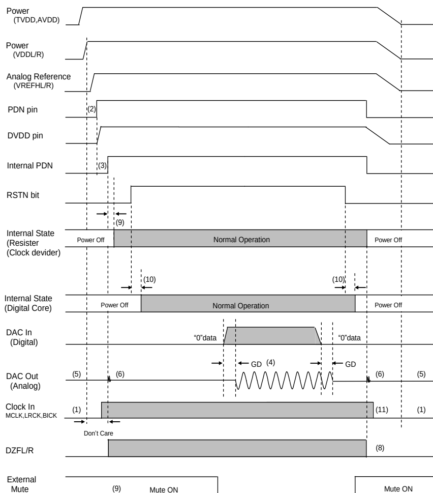
Figure 55. Power-down/up Sequence Example (Resister Control Mode, LDOE pin= "H")
