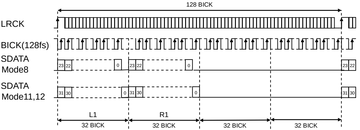
Figure 32. Mode 8/11/12 Timing
