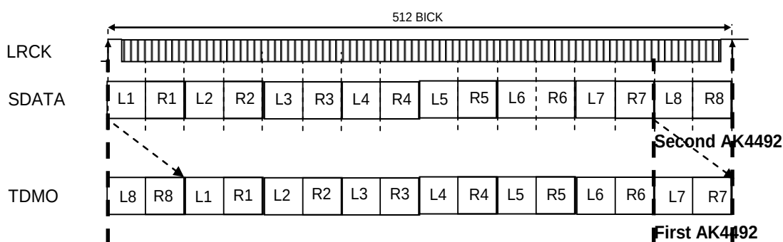
Figure 46. Daisy Chain (TDM512 Mode)
