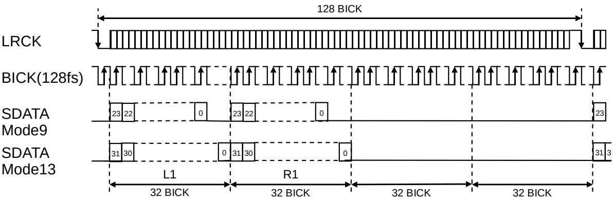
Figure 33. Mode 9/13 Timing
