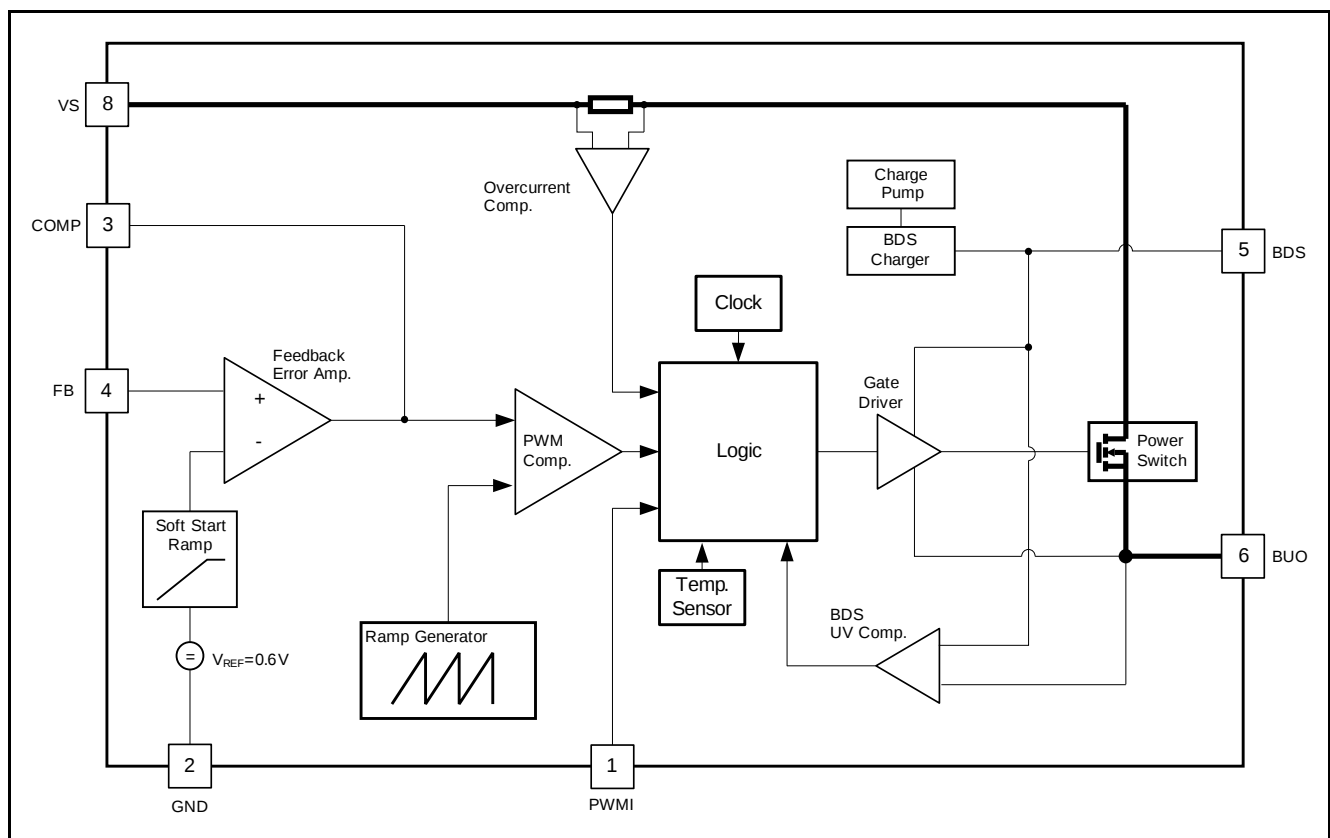
Figure 5-1 Block Diagram Buck Regulator
