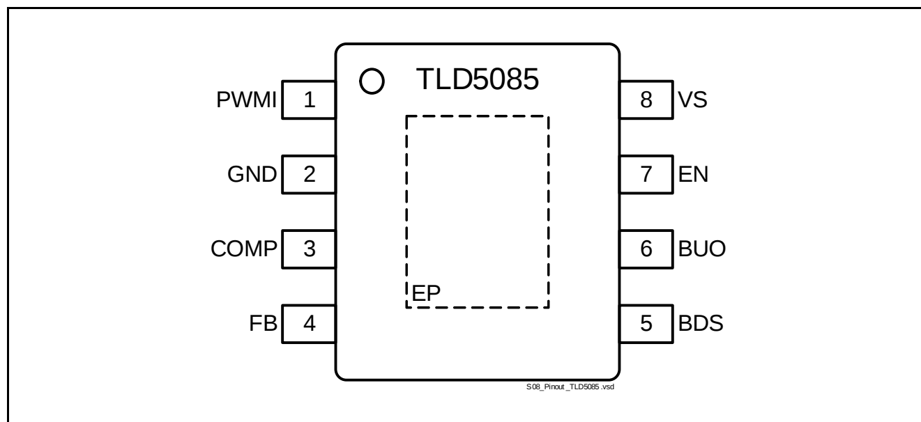
Figure 3-1 Pin Configuration TLD5085EJ
