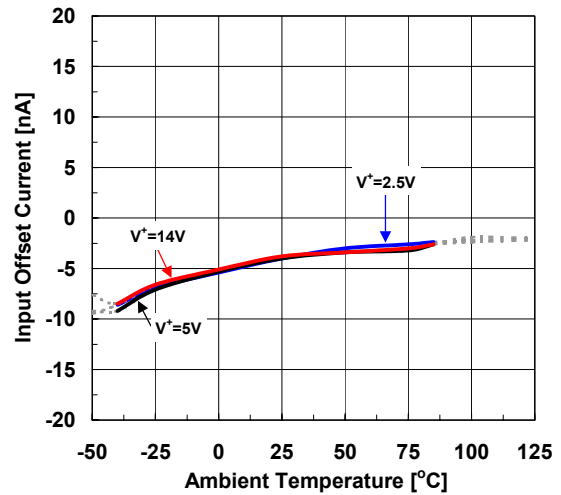
Input Offset Current vs. Ambient Temperature (Supply Voltage) R_L=10k\Omega
