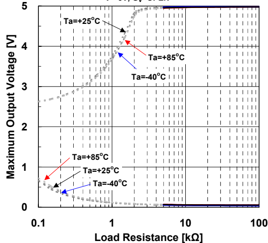
Maximum Output Voltage vs. Load Resistance (Temperature, V^+=5V ) V^+=5V , G_V=OPEN
