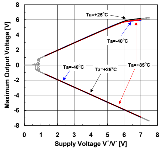
Maximum Output Voltage vs. Supply Voltage (Temperature, R_L=5k\Omega ) G_V=OPEN , R_L=10k\Omega
