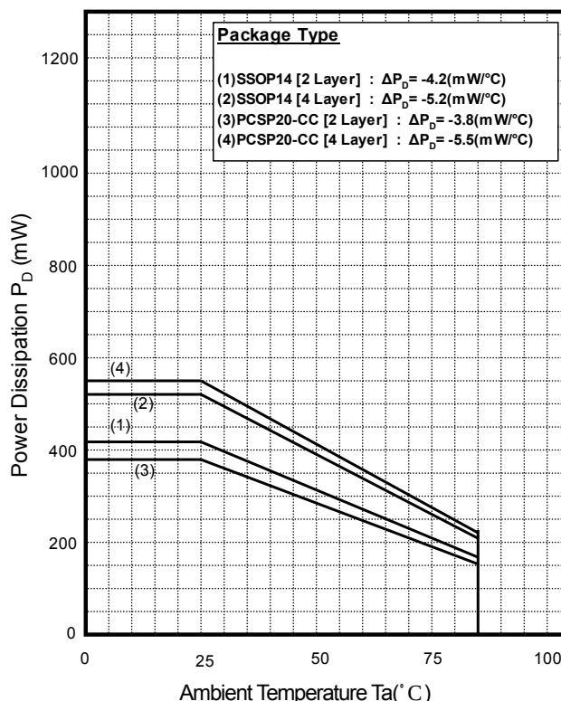
Figure 1B : Power Dissipation – Ambient Temperature
