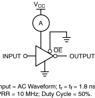
Figure 6. I_{OCD} Test Circuit
