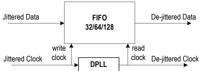
Figure-19 Jitter Attenuator
