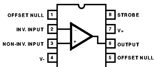
CA5130 (PDIP, SOIC) TOP VIEW
