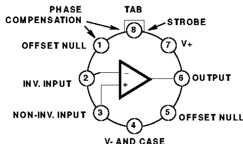
CA5130 (METAL CAN) TOP VIEW
