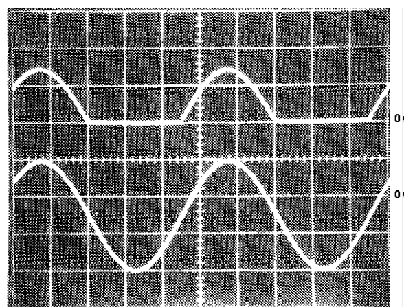
FIGURE 4B. OUTPUT WAVEFORM WITH GROUND REFERENCE SINE WAVE INPUT
