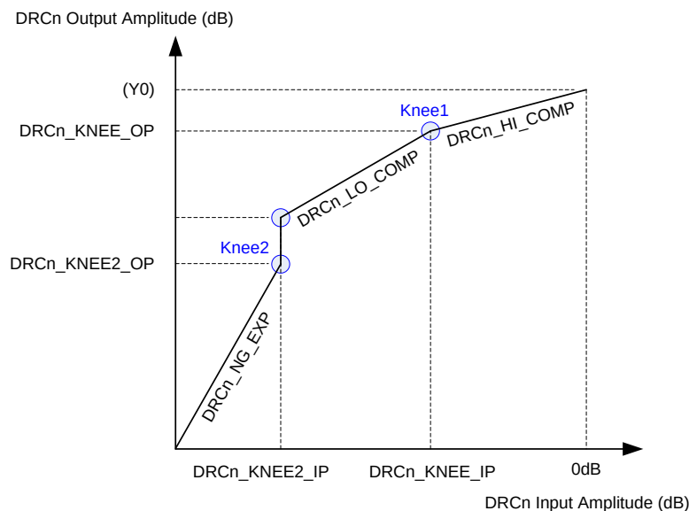
Figure 19 DRC Response Characteristic
