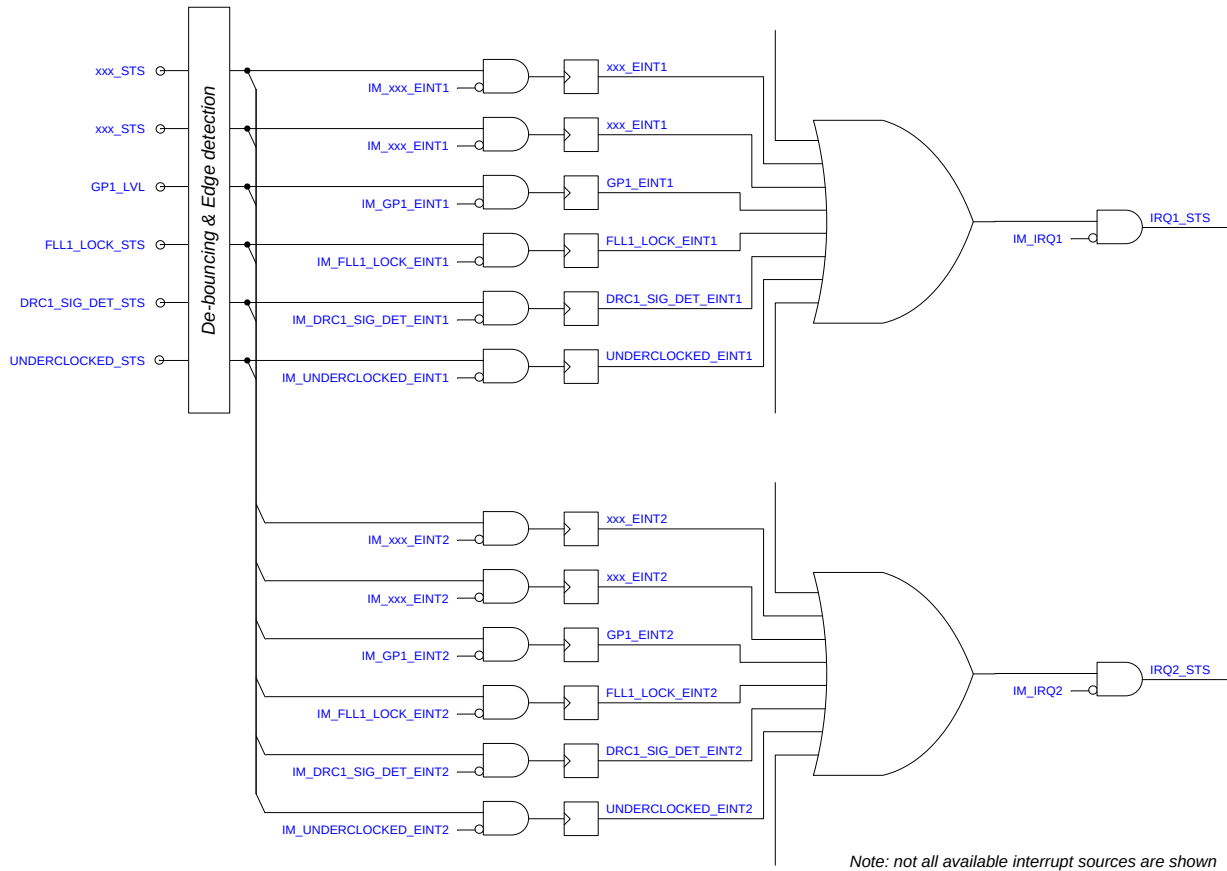
Figure 46 Interrupt Controller
