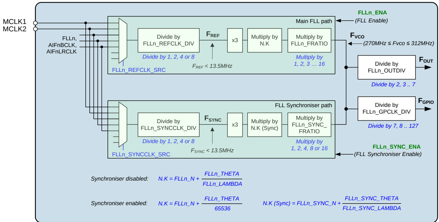
Figure 49 FLL Configuration
