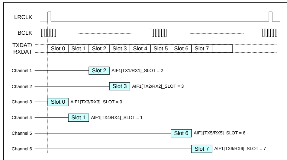
Figure 38 DSP Mode B Example
