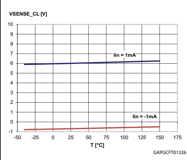
Figure 33. V_{\text{sense clamp}} vs. T_{\text{case}}
