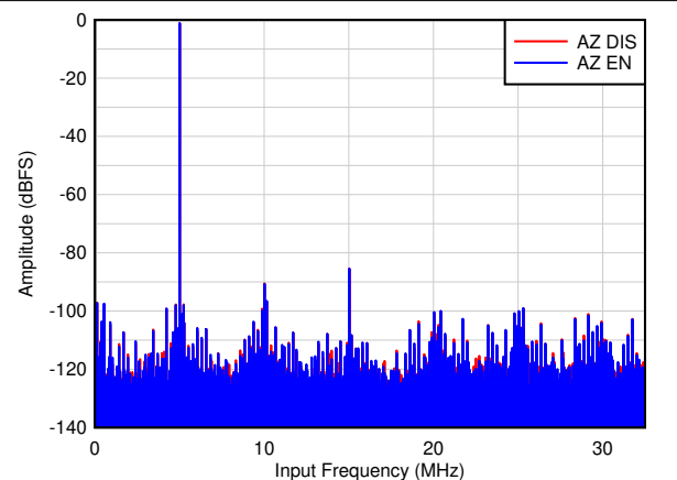
Figure 8-13. F_S = 65 MSPS, F_{IN} = 5 MHz
