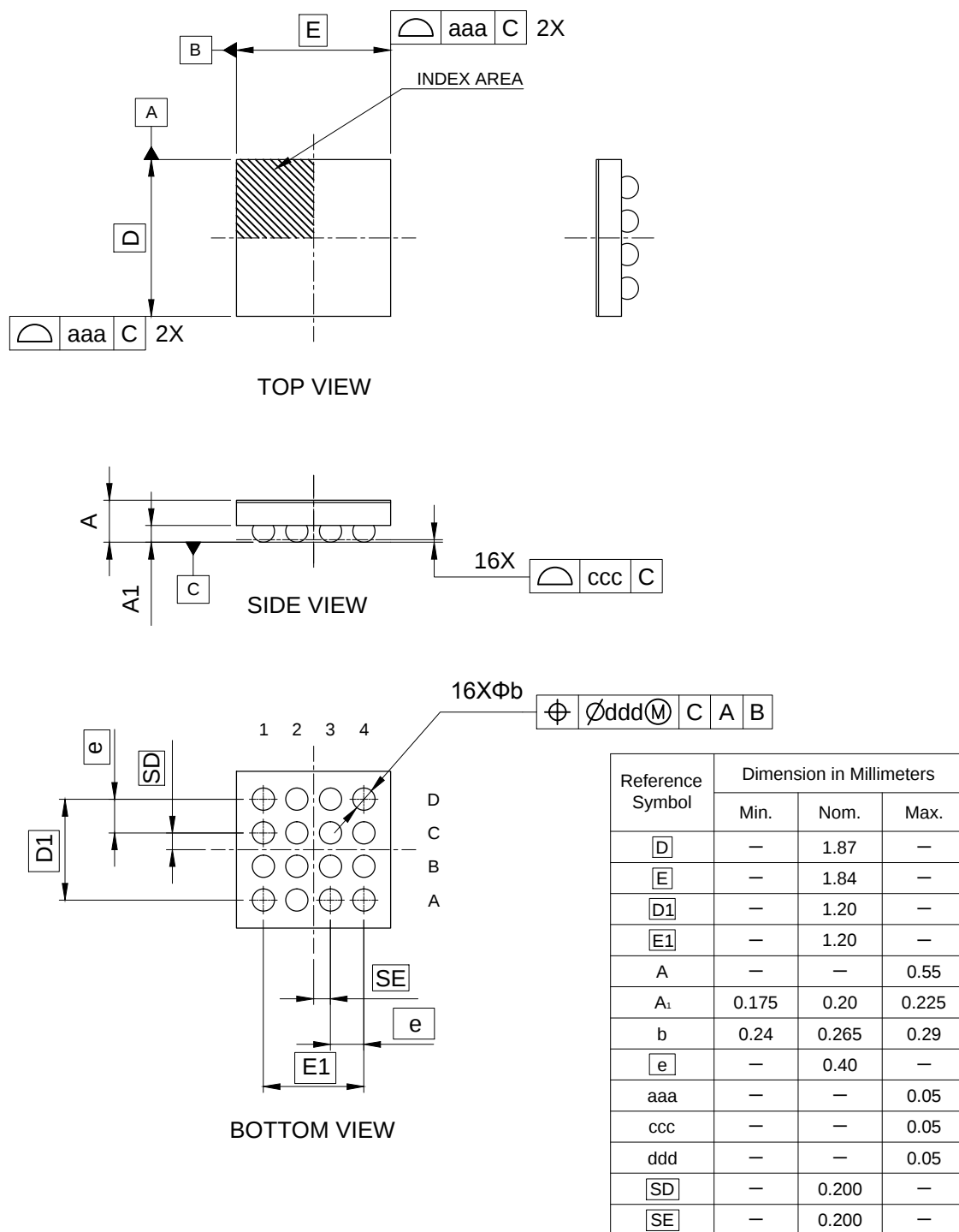
Figure 2.3 WLCSP 16-pin
