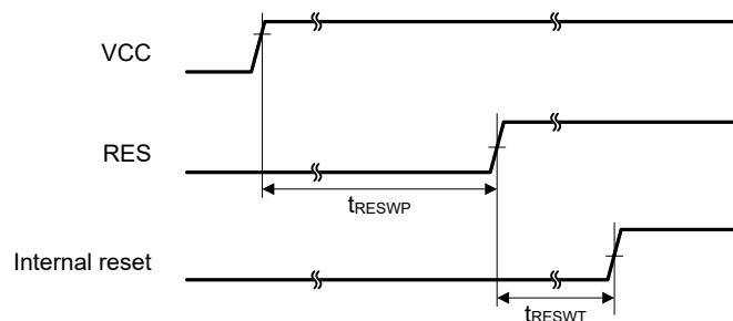
Figure 2.5 Reset input timing at power-on
