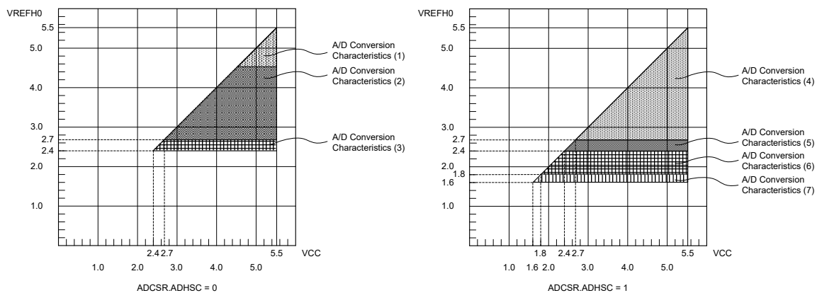
Figure 2.44 AVCC0 to VREFH0 voltage range
