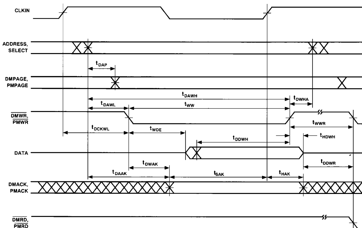
Figure 11. Memory Write
