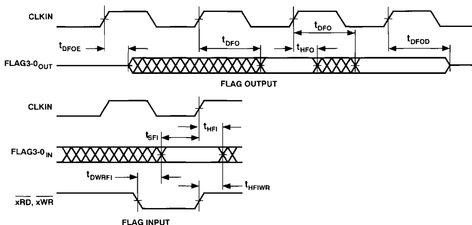
Figure 7. Flags
