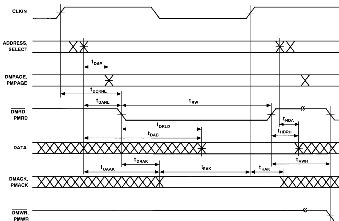
Figure 10. Memory Read
