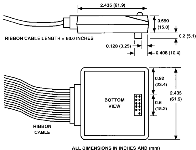
Figure 21. EZ-ICE Probe
