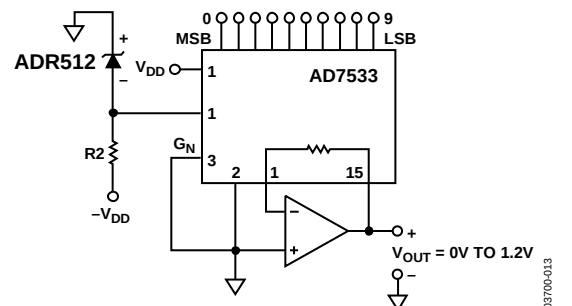
Figure 13. ADR512 as a Reference for a 10-Bit CMOS DAC (AD7533)
