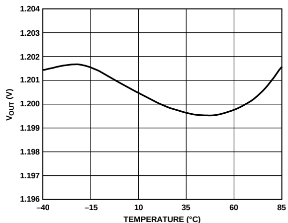
Figure 3. Typical V_{OUT} vs. Temperature
