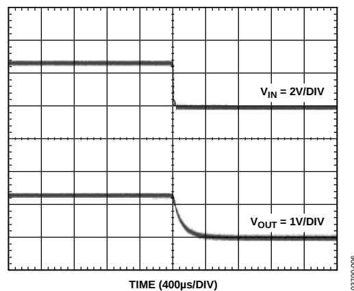
Figure 6. Turn Off Time
