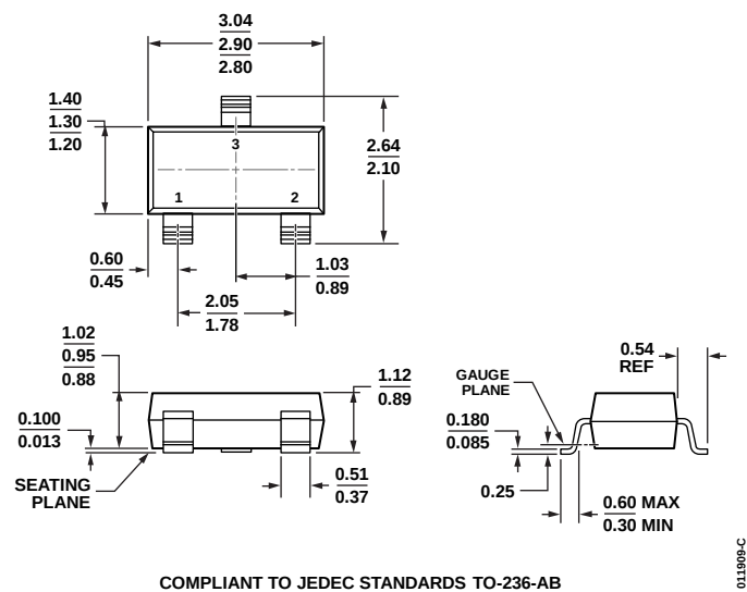
COMPLIANT TO JEDEC STANDARDS TO-236-AB Figure 15. 3-Lead Small Outline Transistor Package [SOT-23] (RT-3) Dimensions shown in millimeters
