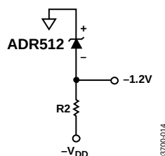
Figure 14. Precise -1.2\text{ V} Reference Configuration
