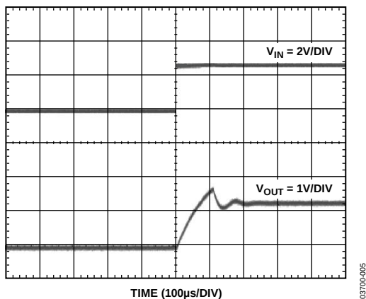
Figure 5. Turn On Time with 1 µF Input Capacitor
