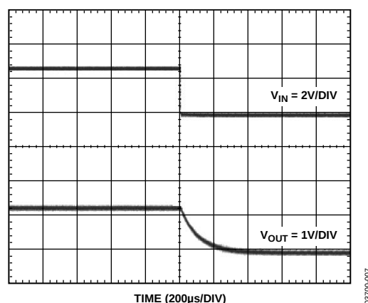
Figure 7. Turn Off Time with 1 µF Input Capacitor
