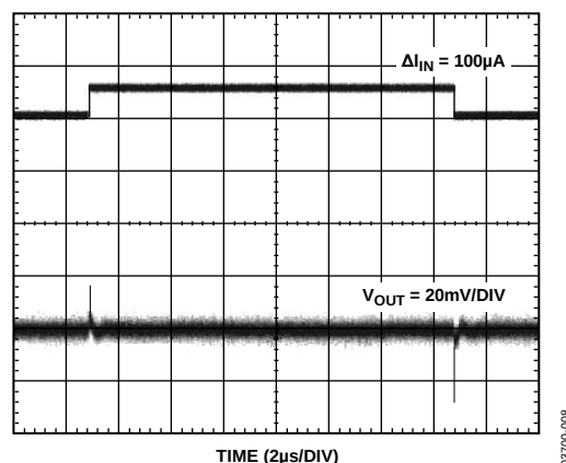
Figure 8. Output Response to 100 µA Input Current Change
